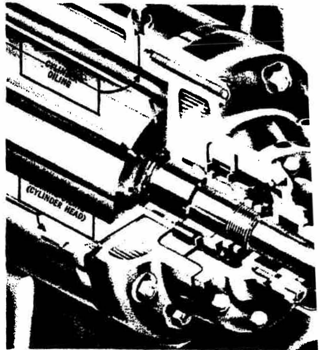
Fig. 11 Force feed oiling to cylinder wall (as shown) on intake quill on other size machines; assures proper oil distribution to all surfaces. Bearing oiling connections on cylinder heads are always located on discharge side.
